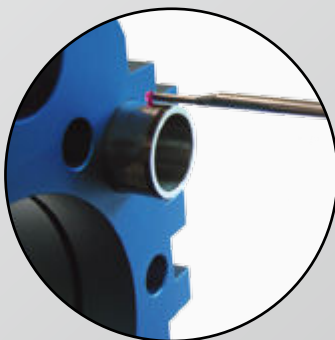
External diameter measurement with the standard probe 930.2101
